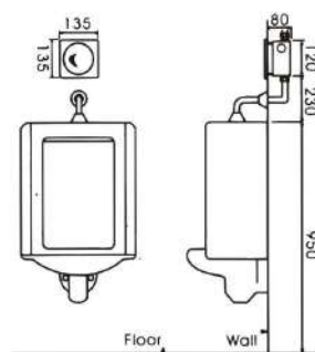
Urinal Flusher with water inlet on the upper side
