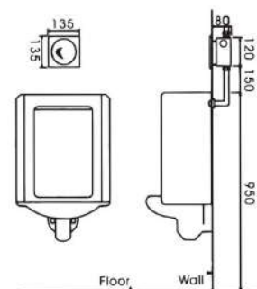
Urinal Flusher with water inlet on the rear side
